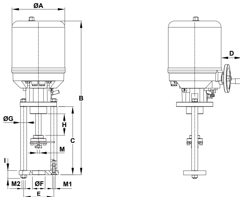
DIMENSIONS (mm)
