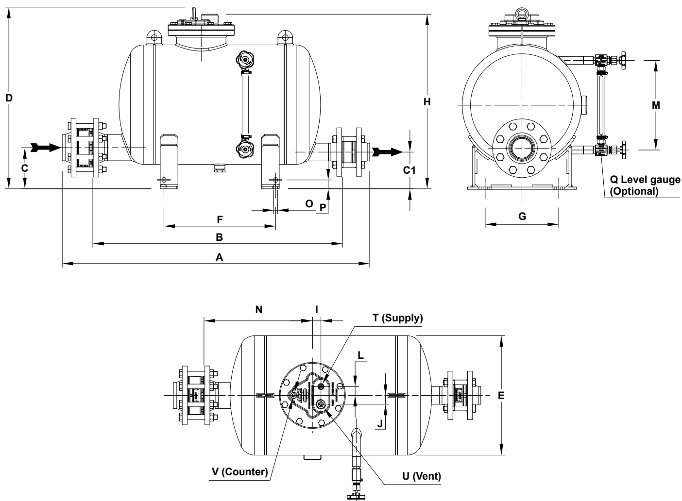
DIMENSIONS (mm)
