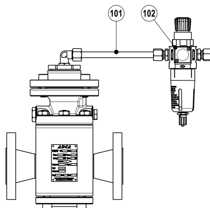
Fig. 5 - Dome loaded valve
