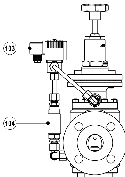
Fig. 7 - Valve with solenoid valve for remote closure
