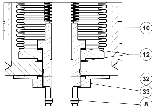
Detail C (DN 125 and DN 150)
