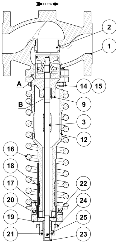
DN 50
