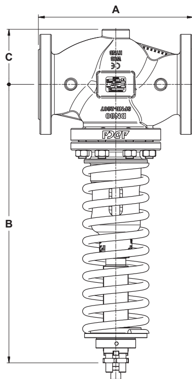
DIMENSIONS – VALVE (mm)
