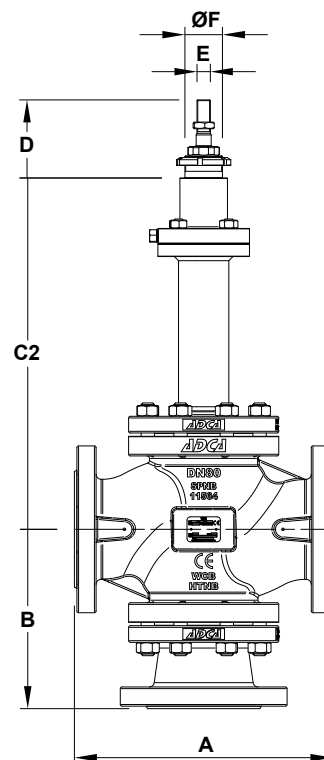
Bellows sealed valve
